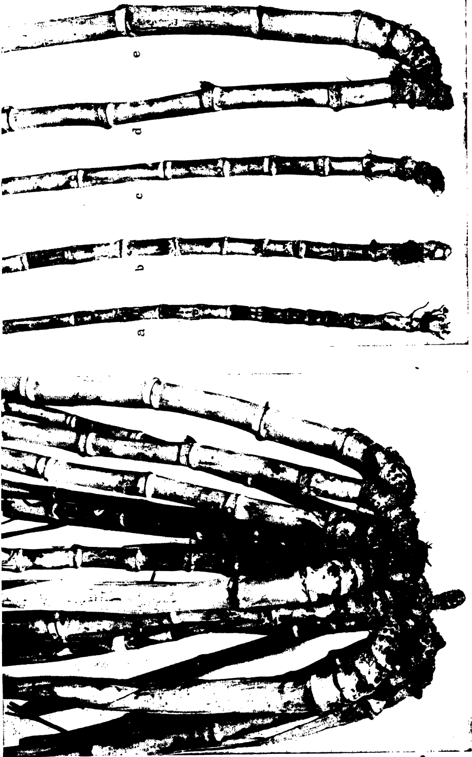
A dissected plant of Pansahi , nine months old, with typical branches of different orders spread out. There is a progressive increase in the length and thickness of the joints and the curvature of the canes, while rooting on the joints becomes less evident. The main stem has a piece of white paper round i
